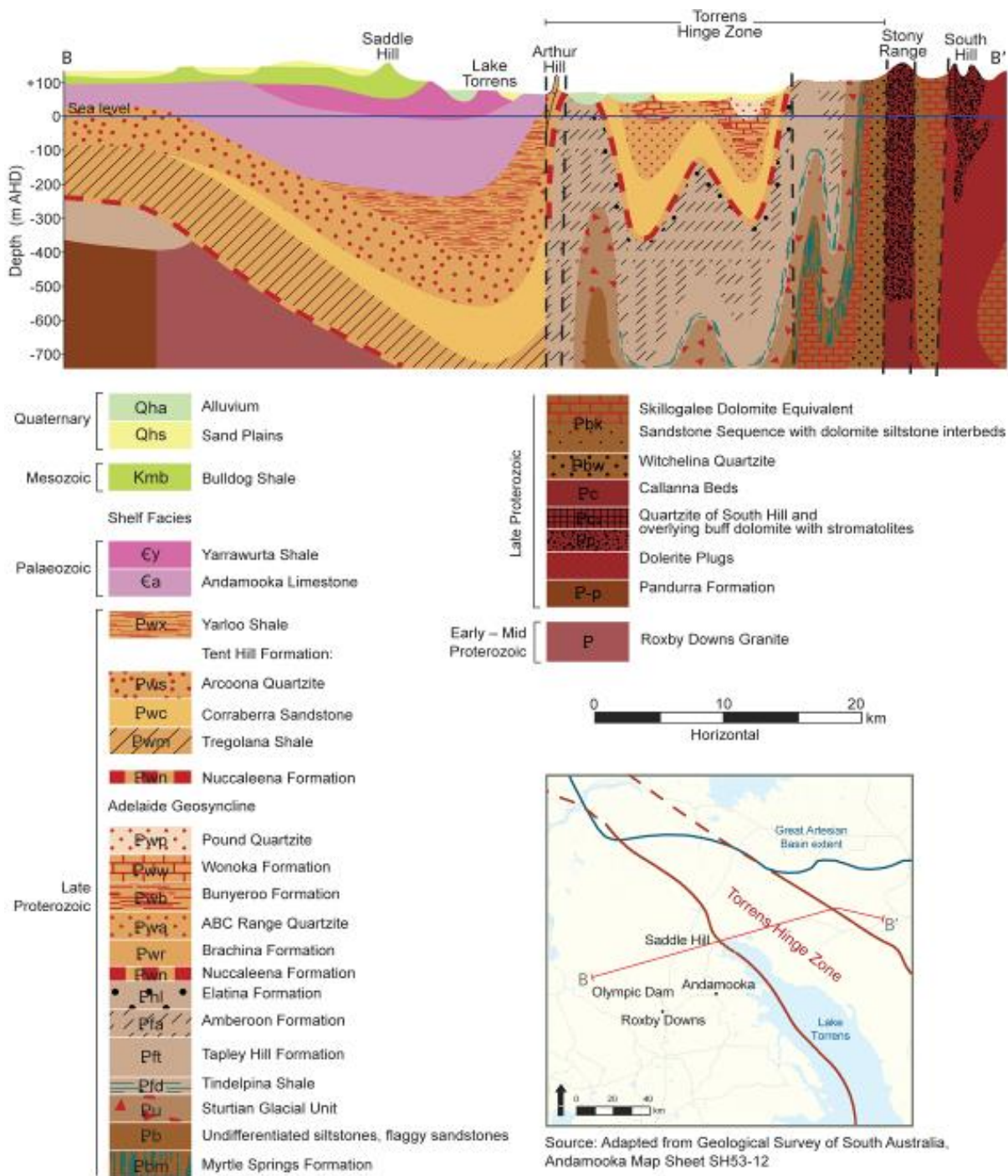
Figure 2-2: Schematic regional geological cross-section
