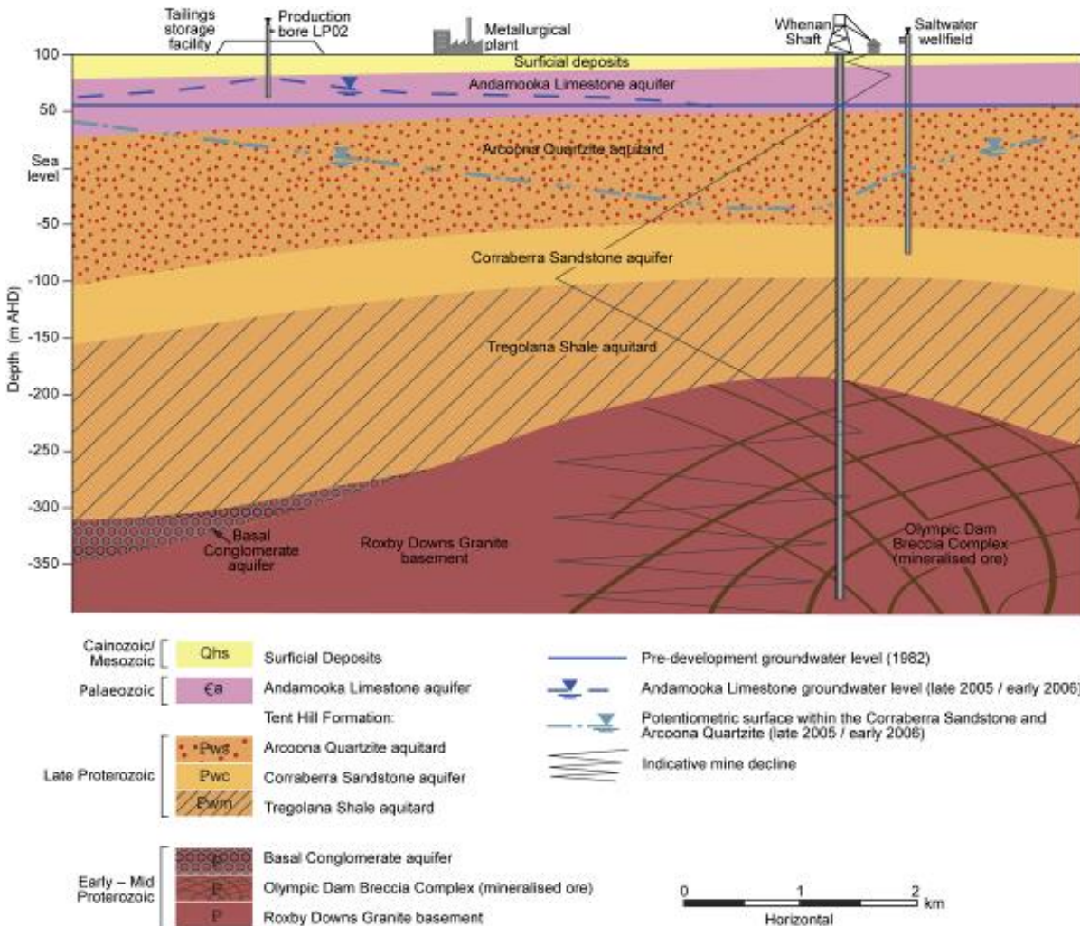
Figure 2-1: Simplified geological cross-section beneath the existing operations
