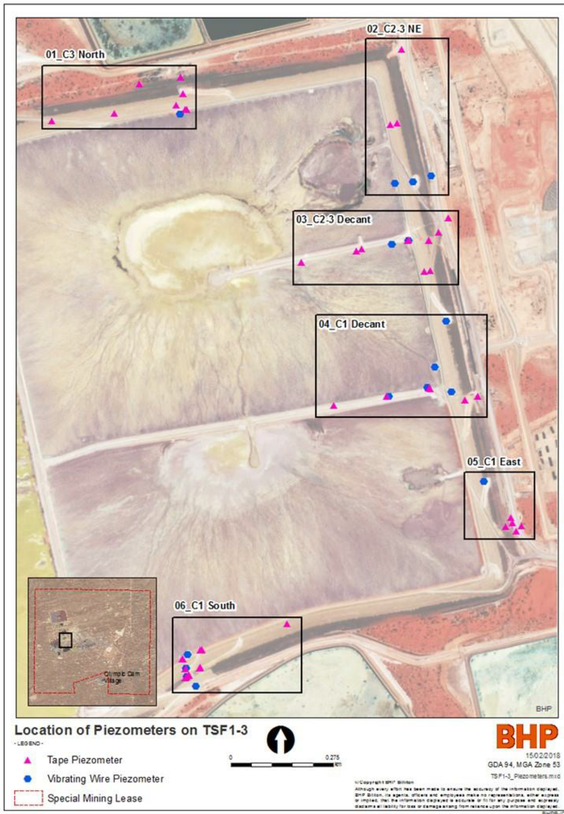
Figure 2-1: Location of piezometers on TSF Cells 1, 2, 3
