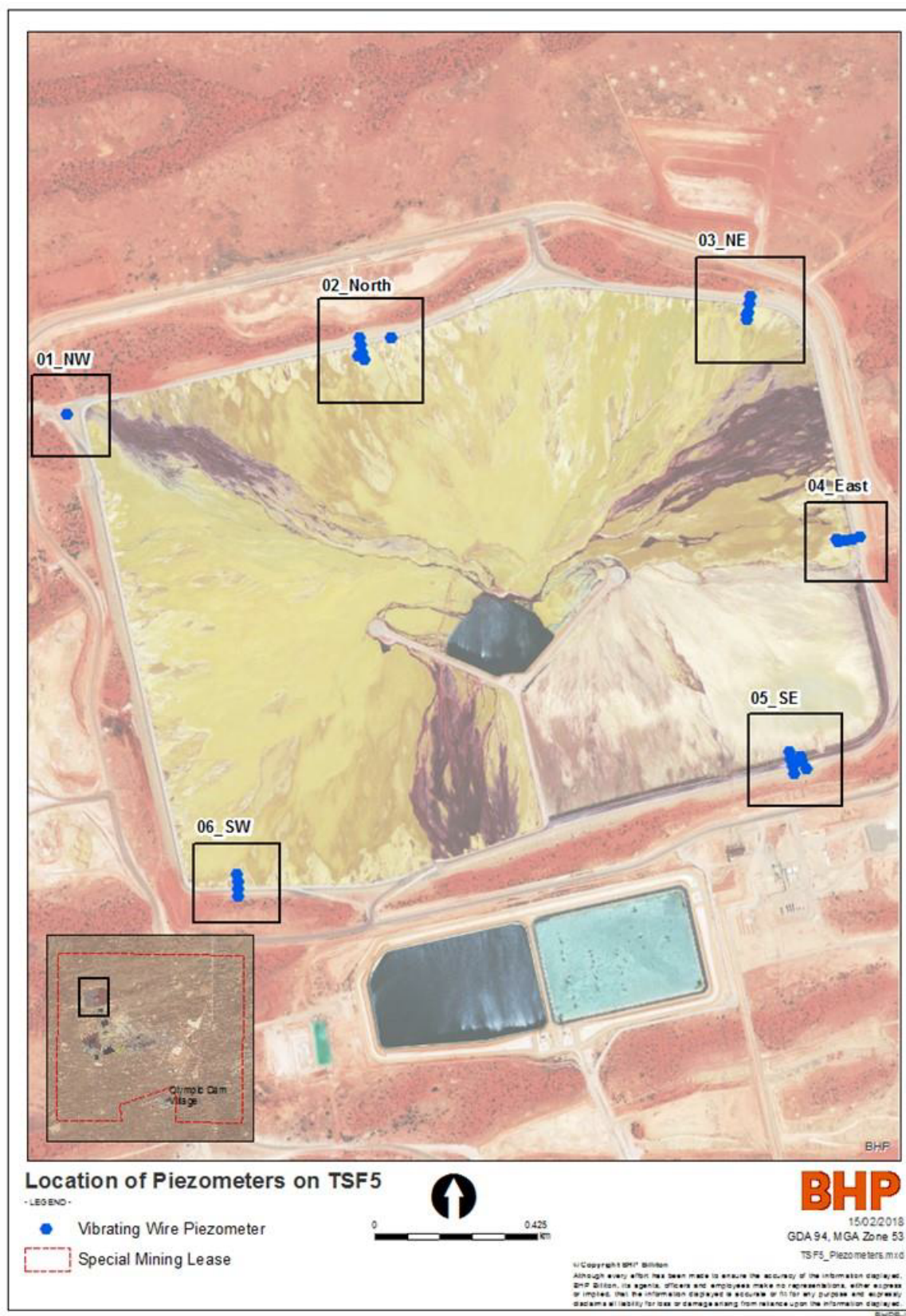
Figure 2-3: Location of piezometers on TSF Cells 5
