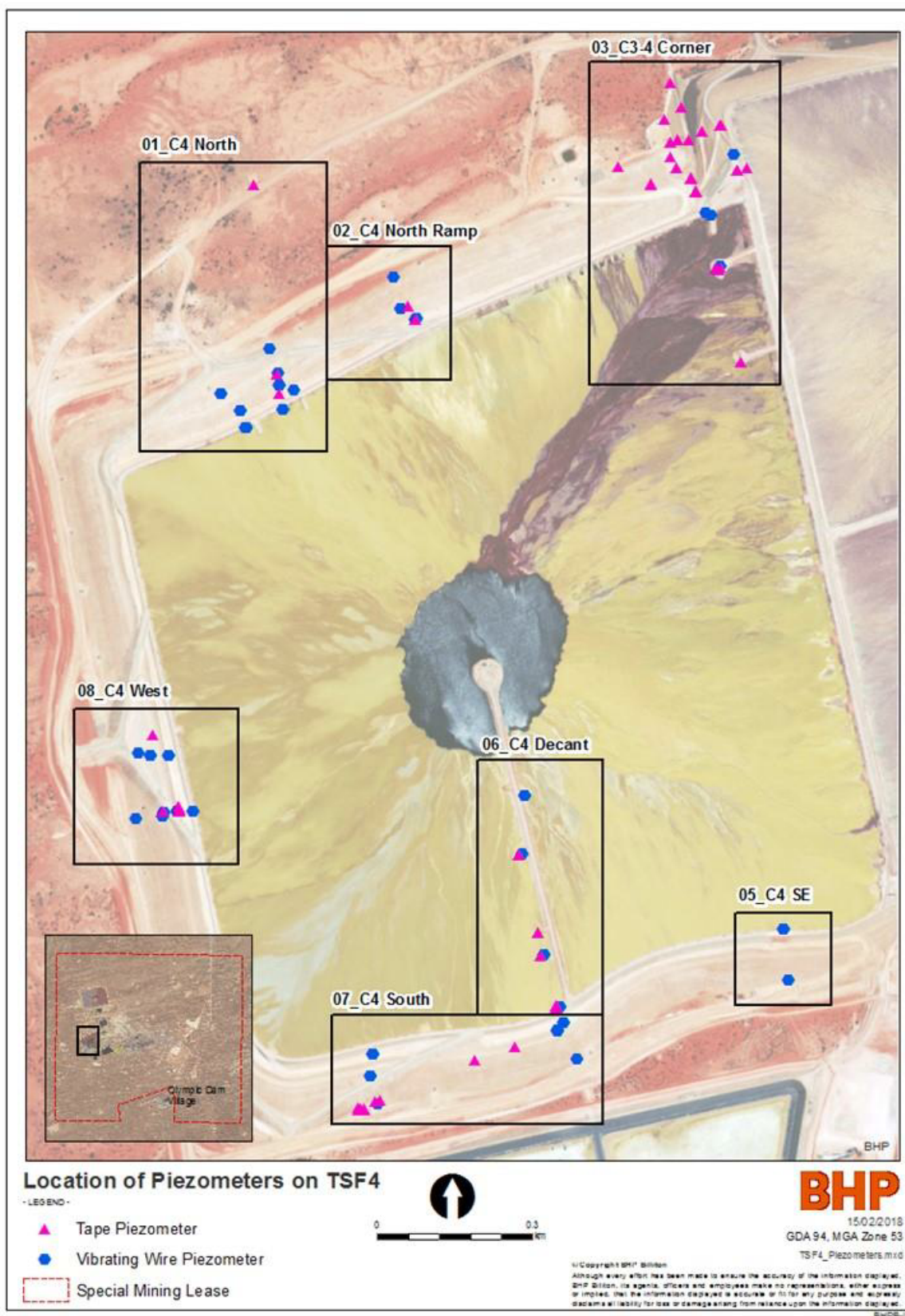
Figure 2-2: Location of piezometers on TSF Cells 4
