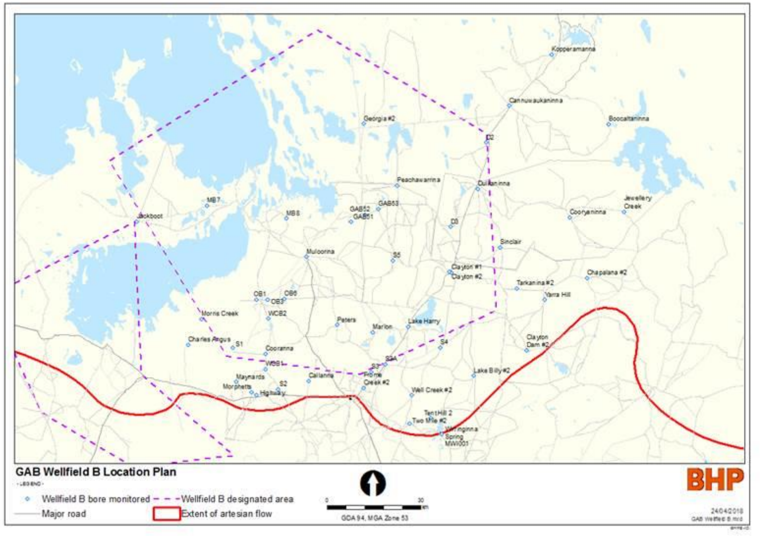
Figure 5.2: GAB Wellfield B location plan
