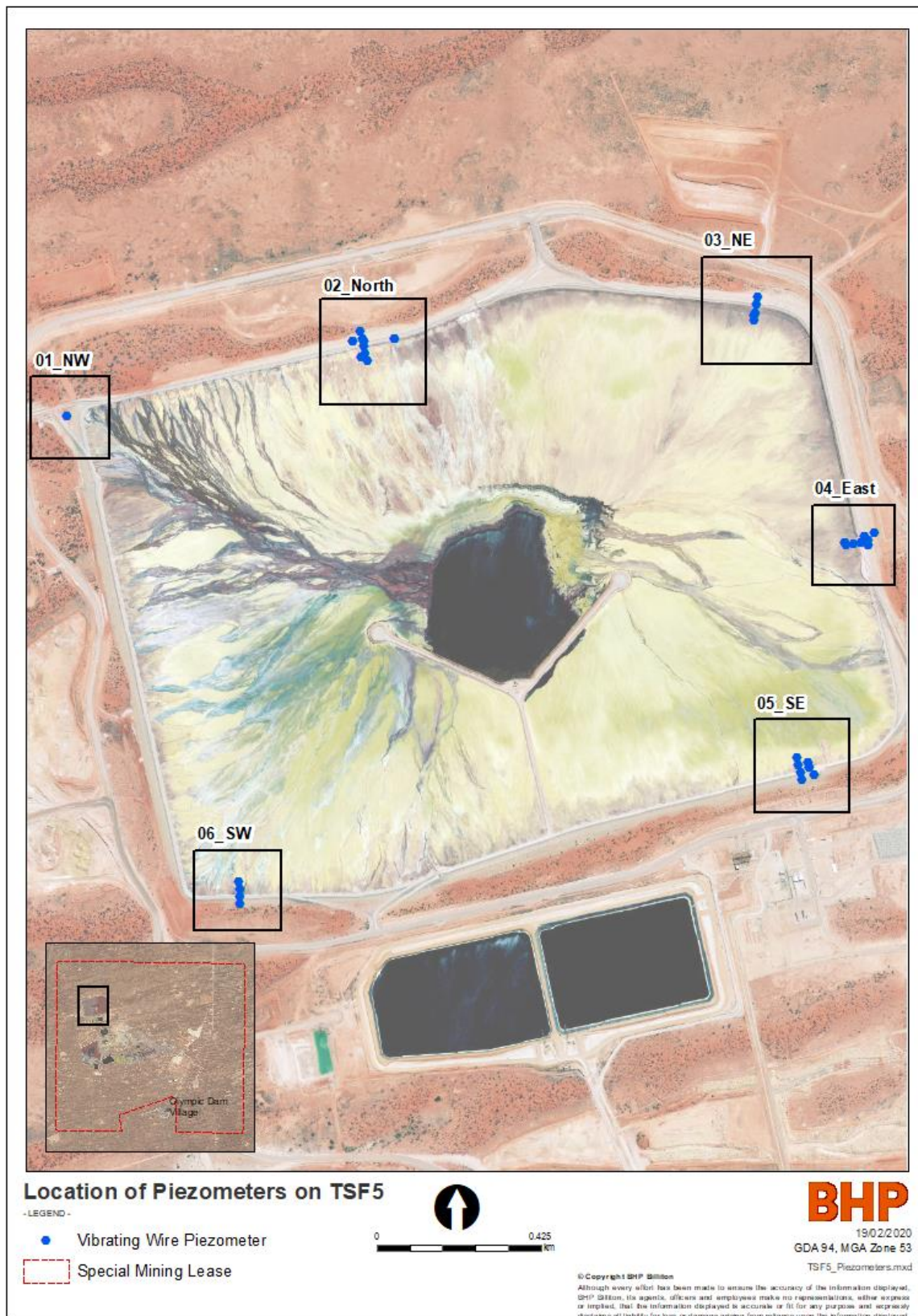
Figure 2-3: Location of piezometers on TSF Cell 5
