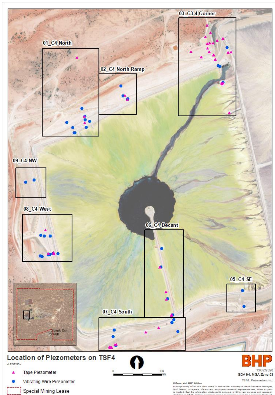
Figure 2-2: Location of piezometers on TSF Cell 4
