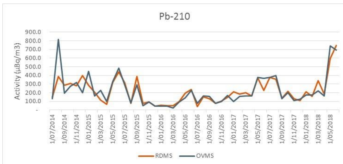
Figure 60: ^{210}\text{Pb} concentration for the 5 year period FY14-FY18 (PM10)
