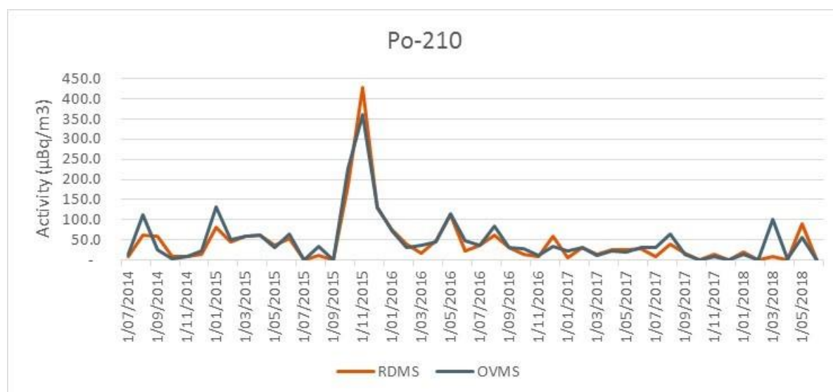
Figure 61: 210 Po concentration for the 5 year period FY14-FY18 (PM10)
