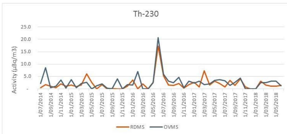
Figure 58: ^{230}\text{Th} concentration for the 5 year period FY14-FY18 (PM10)
