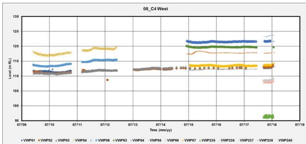
Figure 72: TSF 4 West Wall VWP readings
