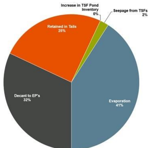
Figure 76: TSF Cells 4 & 5 Liquor Balance – Outputs, FY18
