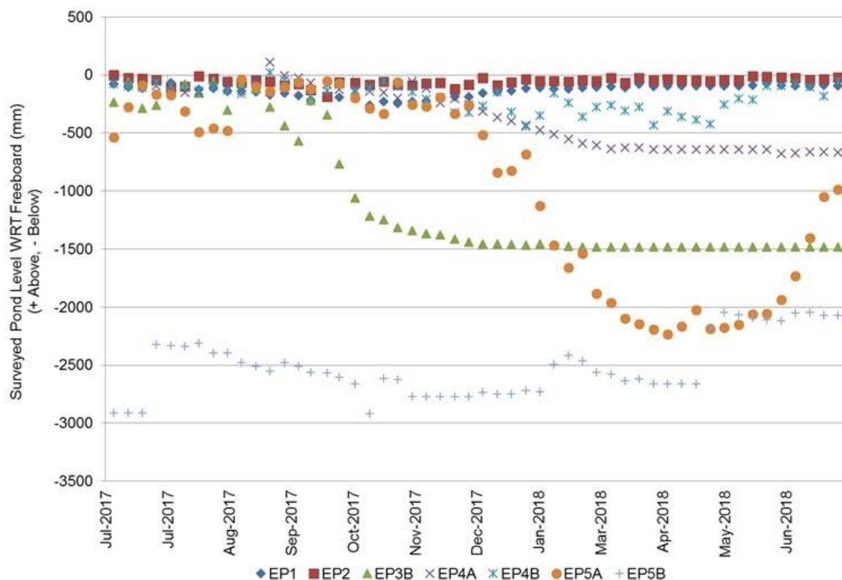
Figure 77: Evaporation Pond Liquor Levels.
