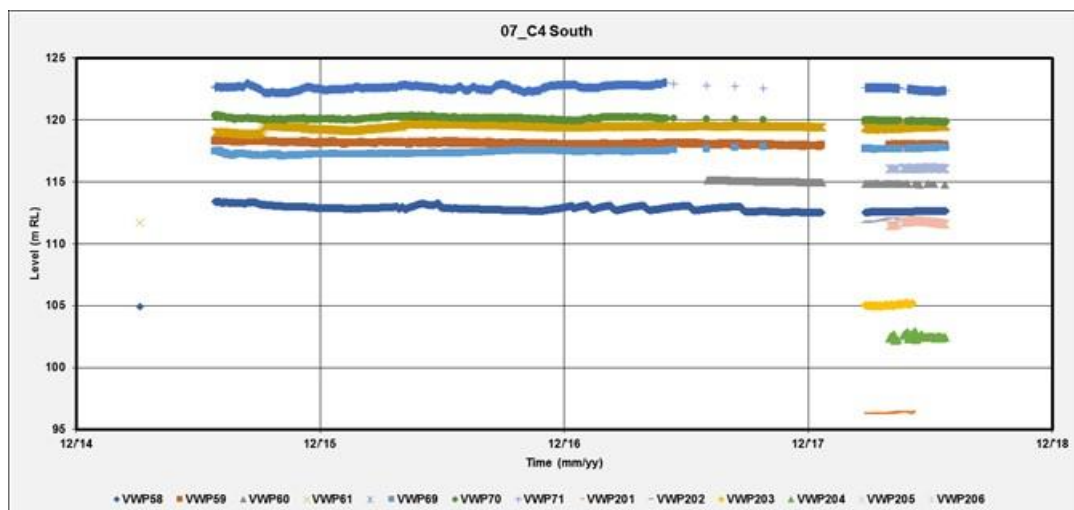
Figure 71: TSF 4 South Wall VWP readings
