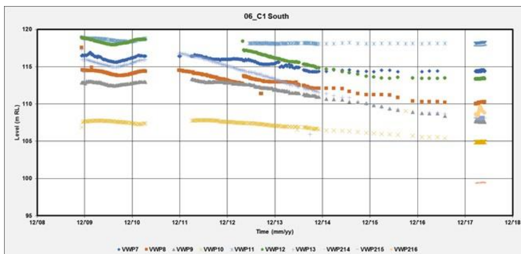
Figure 70: TSF 1 South Wall VWP readings
