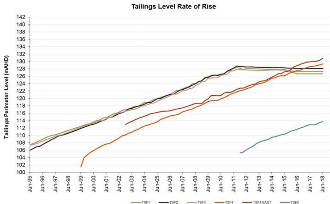
Figure 65: TSF rate of tailings rise.
