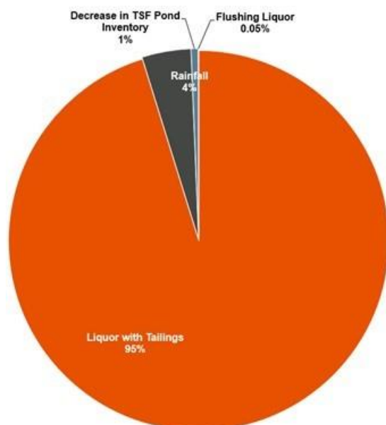
Figure 75: TSF Cells 4 & 5 Liquor Balance – Inputs FY18
