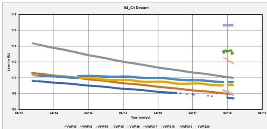
Figure 69: TSF 1 East Wall VWP readings
