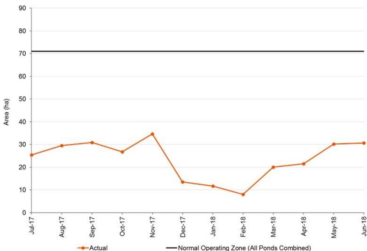
Figure 64: TSF Pond areas (ha) for FY18.
