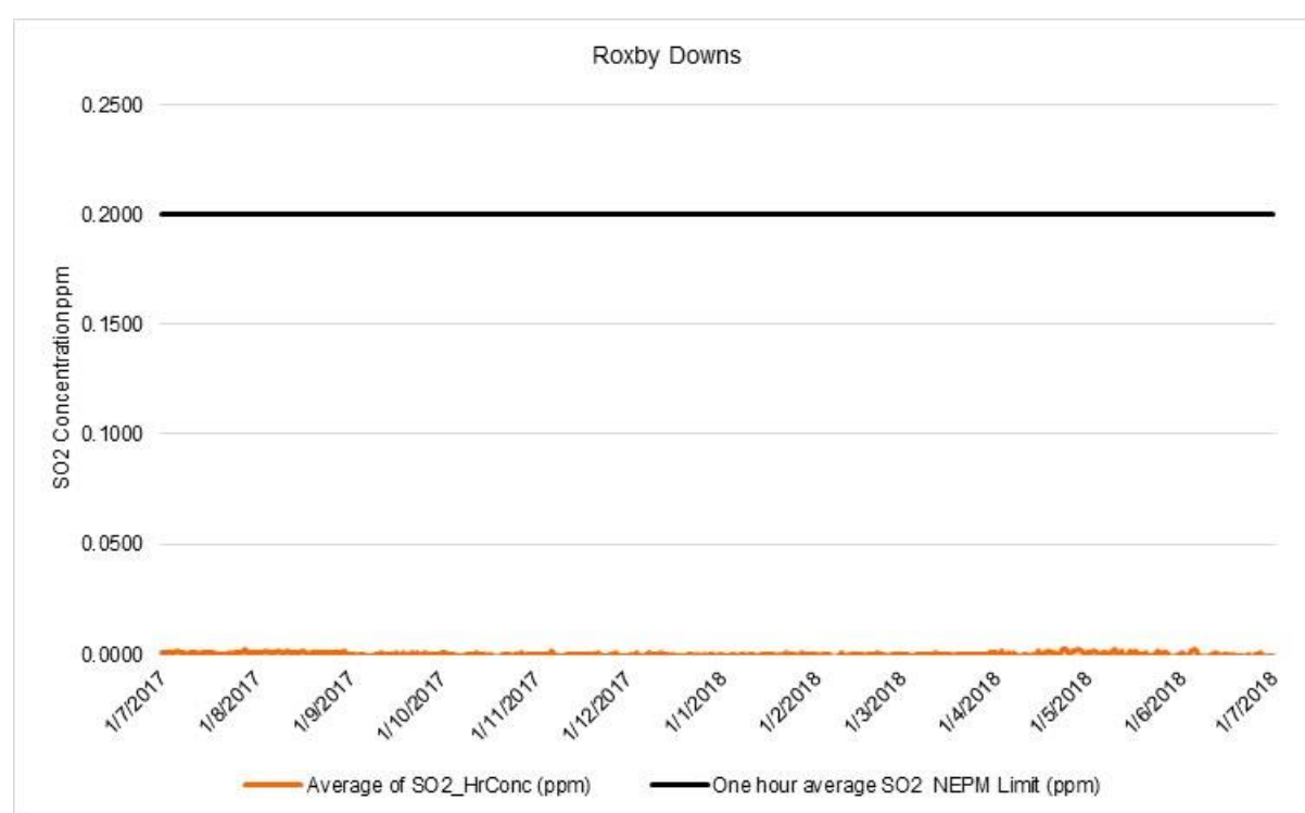
Figure 48: Measured hourly mean SO 2 concentration at sensitive receptor, Roxby Downs.
