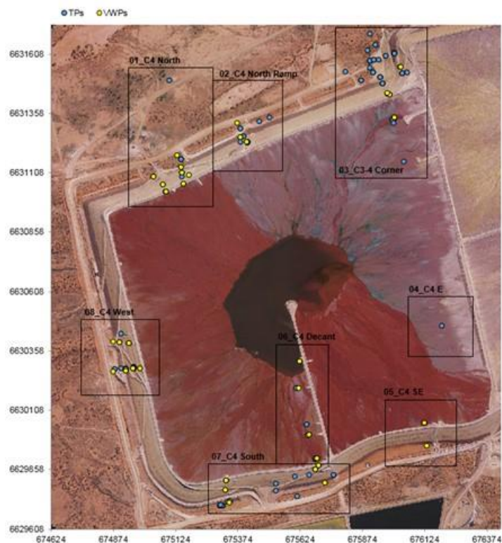
Figure 67: TSF 4 piezometer locations
