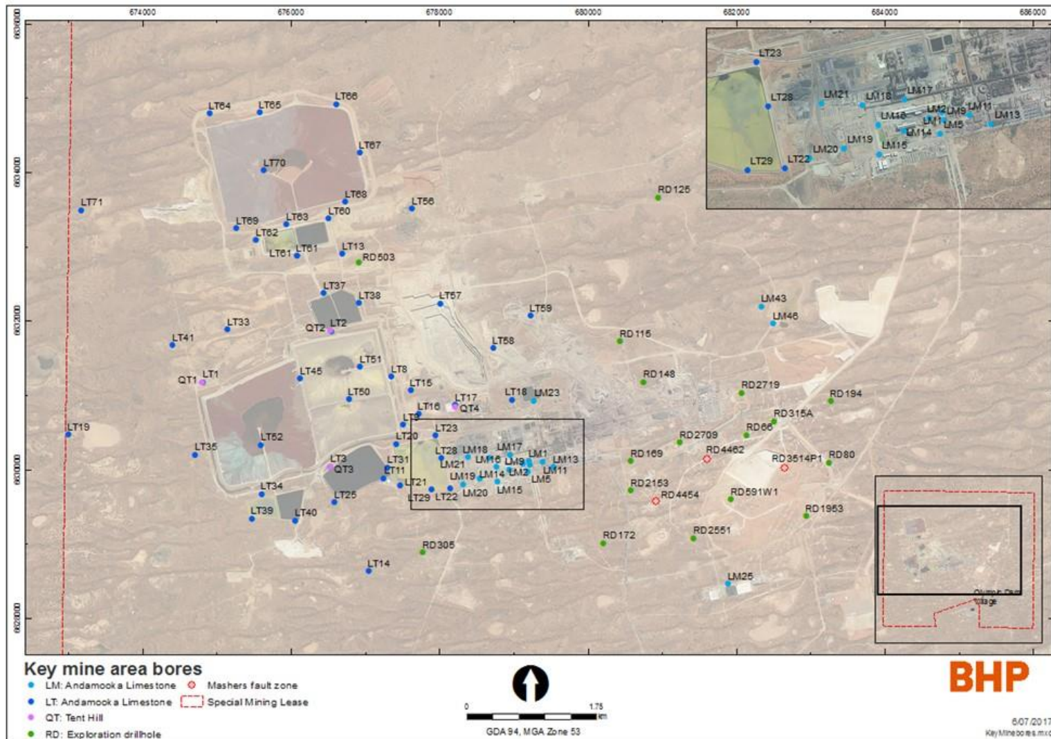
Figure 28: Location of key mine area bores.
