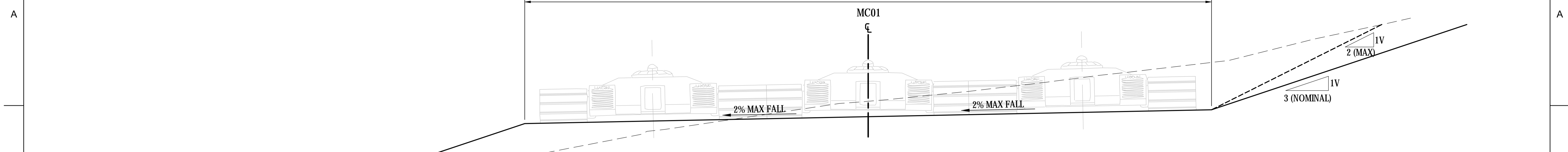
TYPICAL SECTION TYPE 3 - DRAGLINE WALK FORMATION STEEP TERRAIN SCALE 1:100
