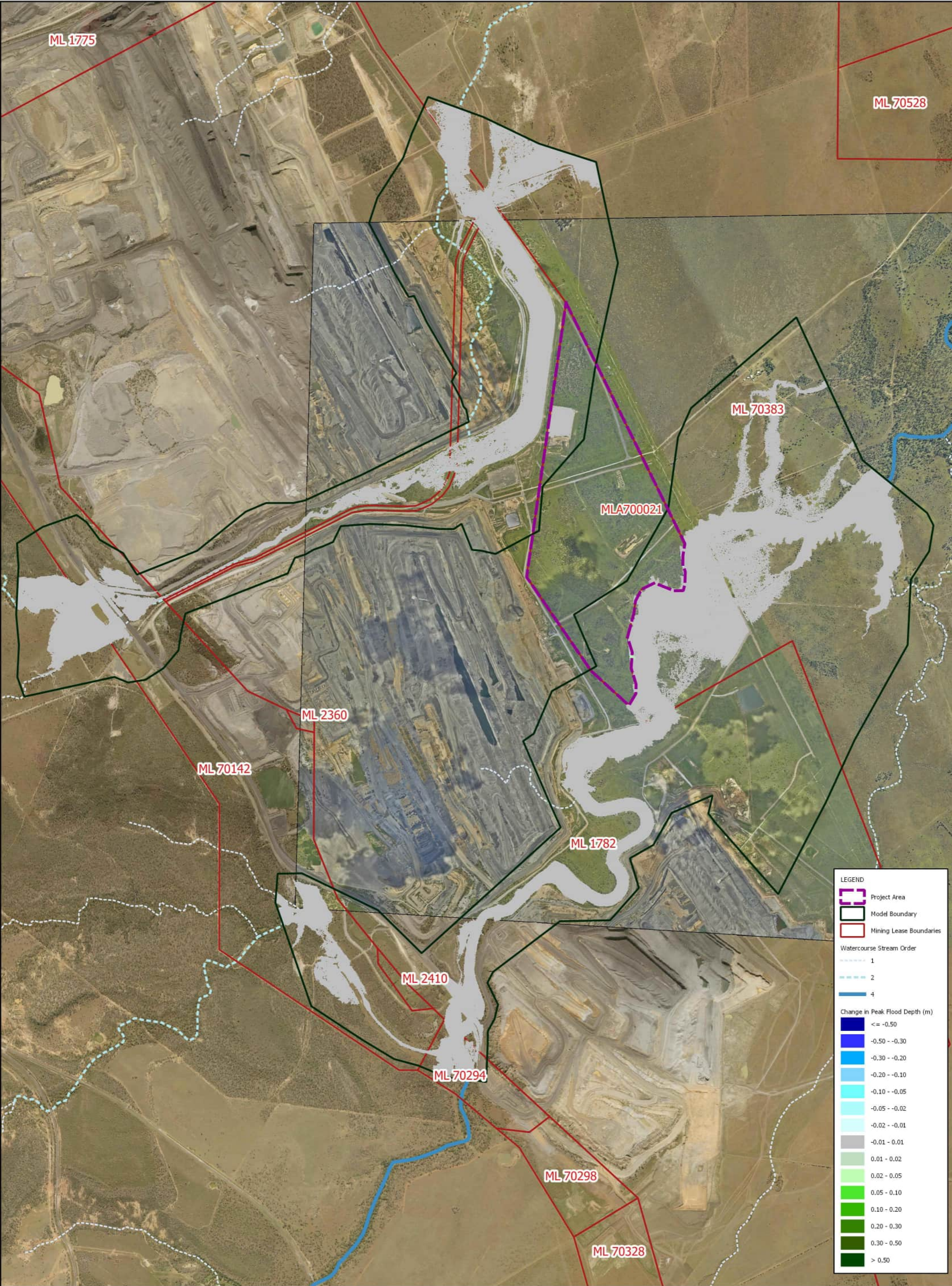
Figure 11 BM Alliance Coal Operations Pty Ltd Saraji Mine Grevillea Pit Continuation Project Surface Water Assessment Change in 1% AEP Flood Depth Drg Ref.
