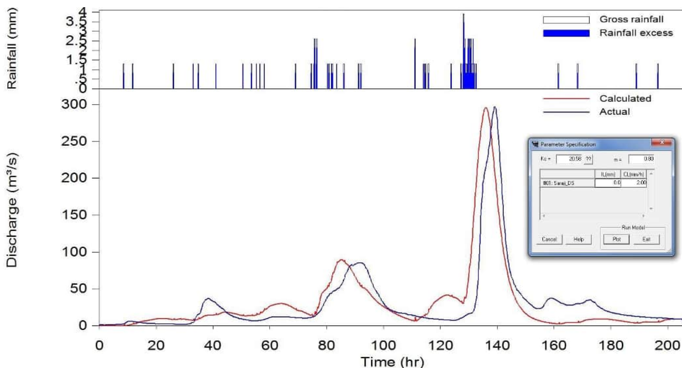
Figure 6.4: Comparison of Modelled and Recorded Flows at Saraji Downstream, December 2010 Event
