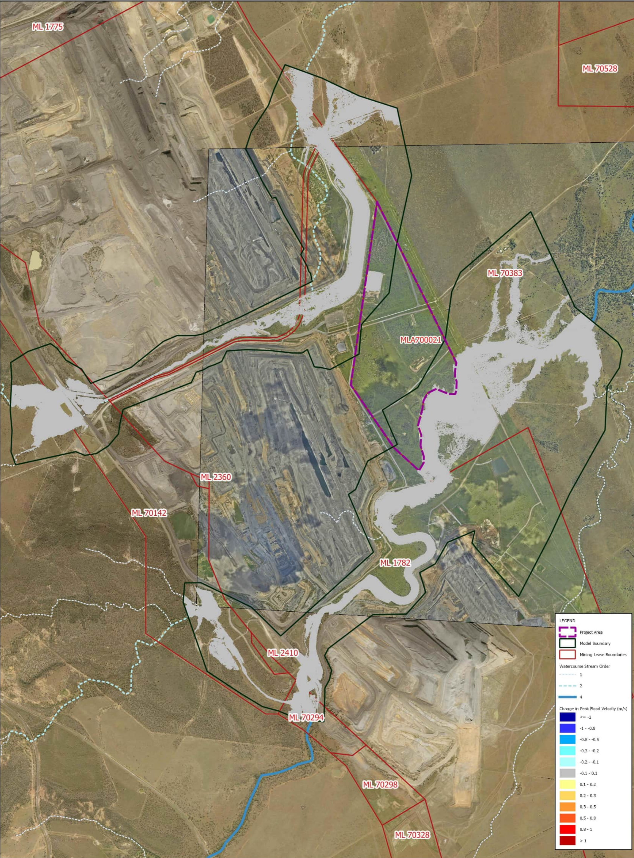
Figure 12 BM Alliance Coal Operations Pty Ltd Saraji Mine Grevillea Pit Continuation Project Surface Water Assessment Change in 1% AEP Flood Velocity Drg Ref.
