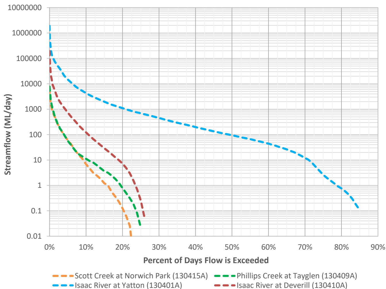
Figure 2.7: Flow Duration Curves
