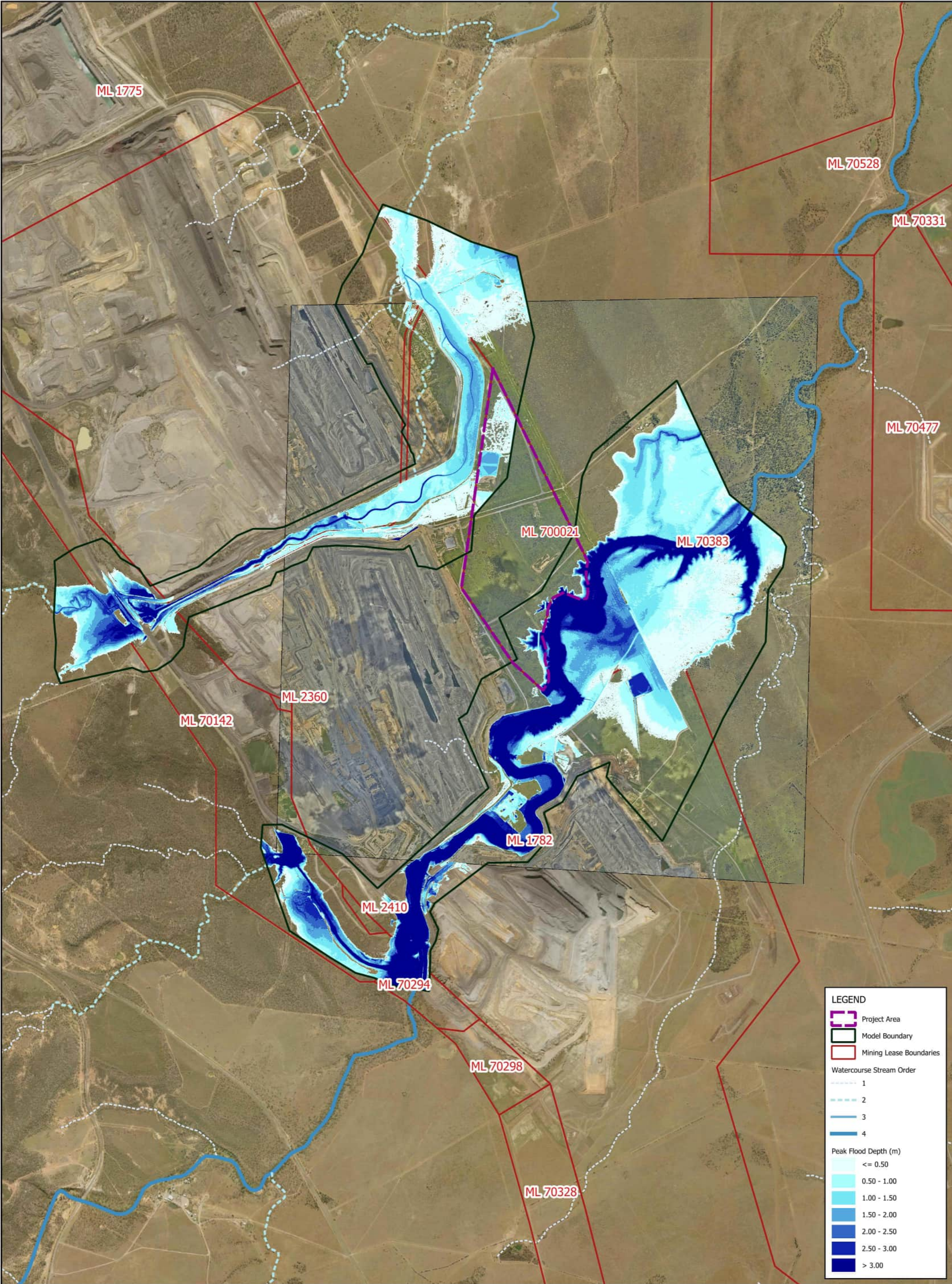
Figure 3 BM Alliance Coal Operations Pty Ltd Saraji Mine Grevillea Pit Continuation Project Surface Water Assessment Base Case 0.1% AEP Flood Depth Climate Change Sensitivity (SSP2-4.5) Drg Ref.
