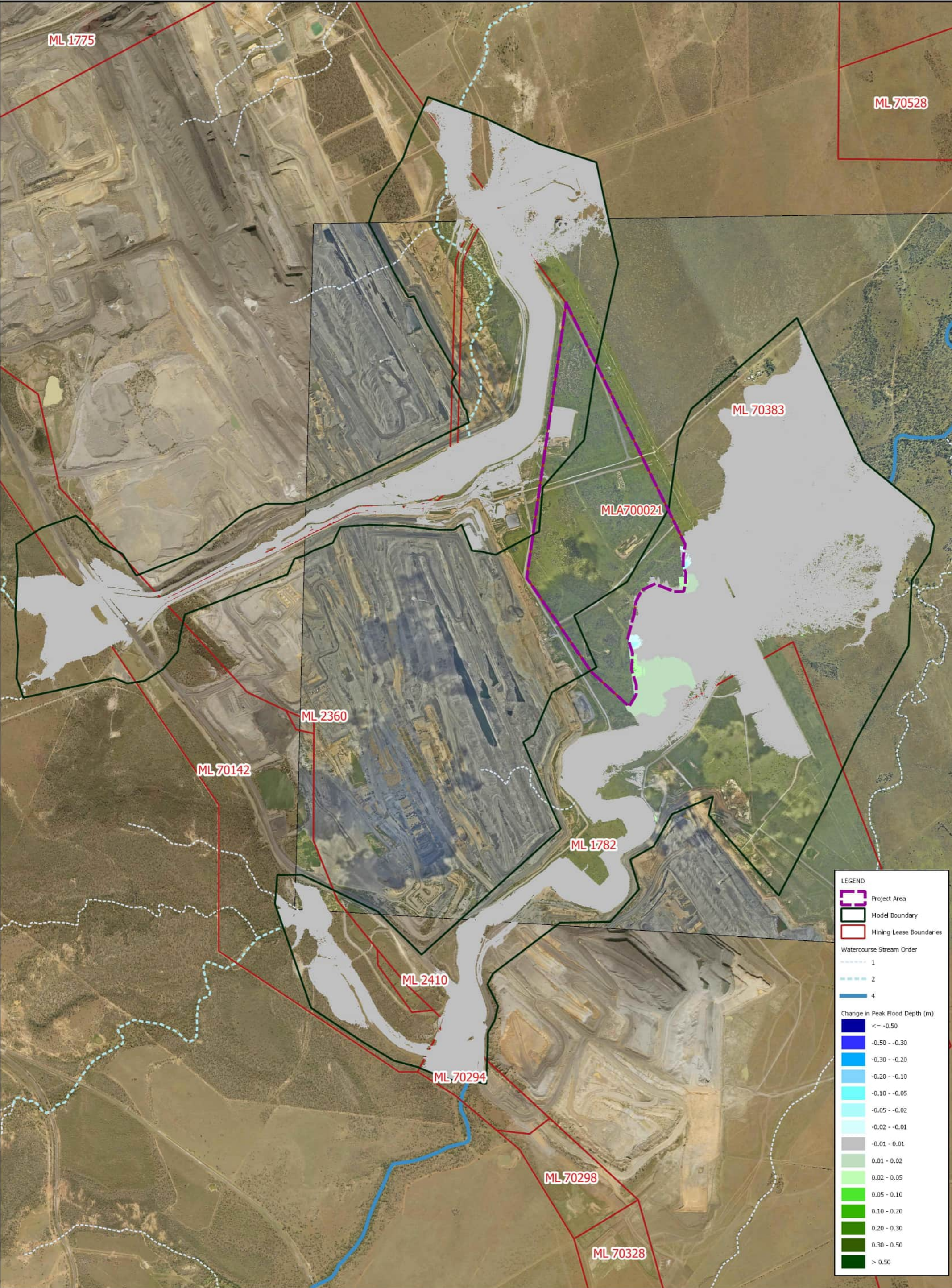
Figure 13 BM Alliance Coal Operations Pty Ltd Saraji Mine Grevillea Pit Continuation Project Surface Water Assessment Change in 0.1% AEP Flood Depth Drg Ref.
