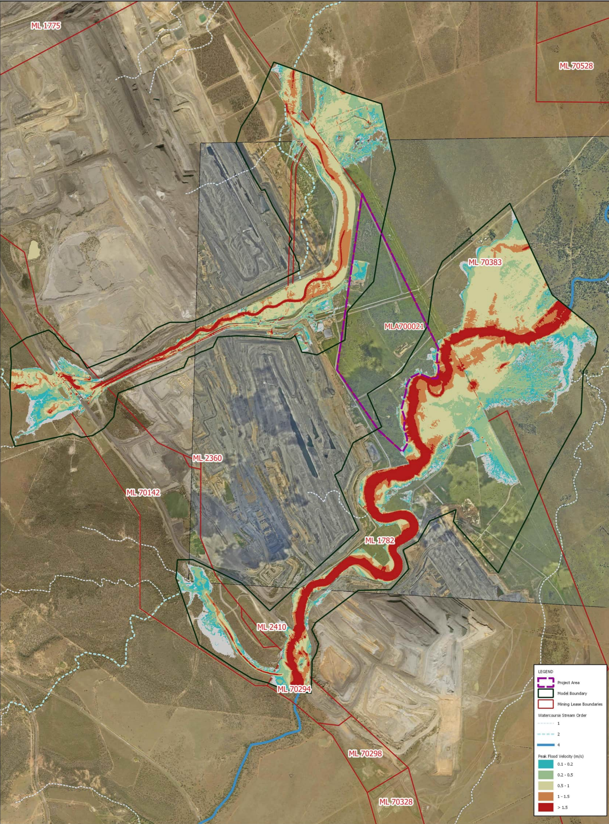
Figure 6 BM Alliance Coal Operations Pty Ltd Saraji Mine Grevillea Pit Continuation Project Surface Water Assessment Base Case 0.1% AEP Flood Velocity Drg Ref.
