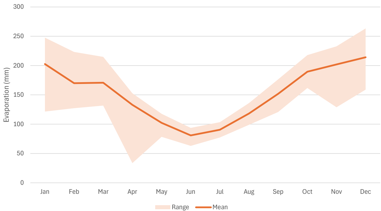
Figure 2.4: Monthly Evaporation
