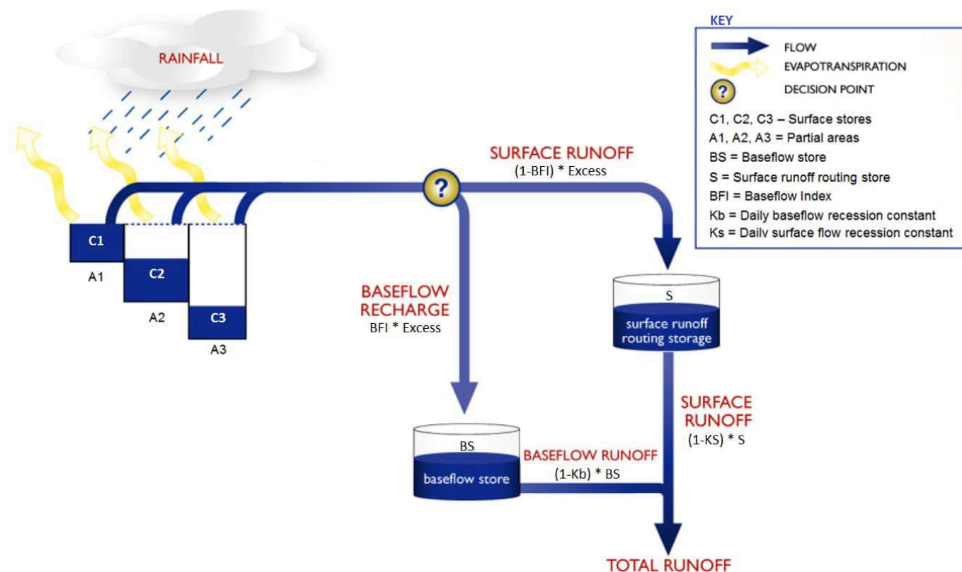
Figure 5.2: AWBM Schematic
