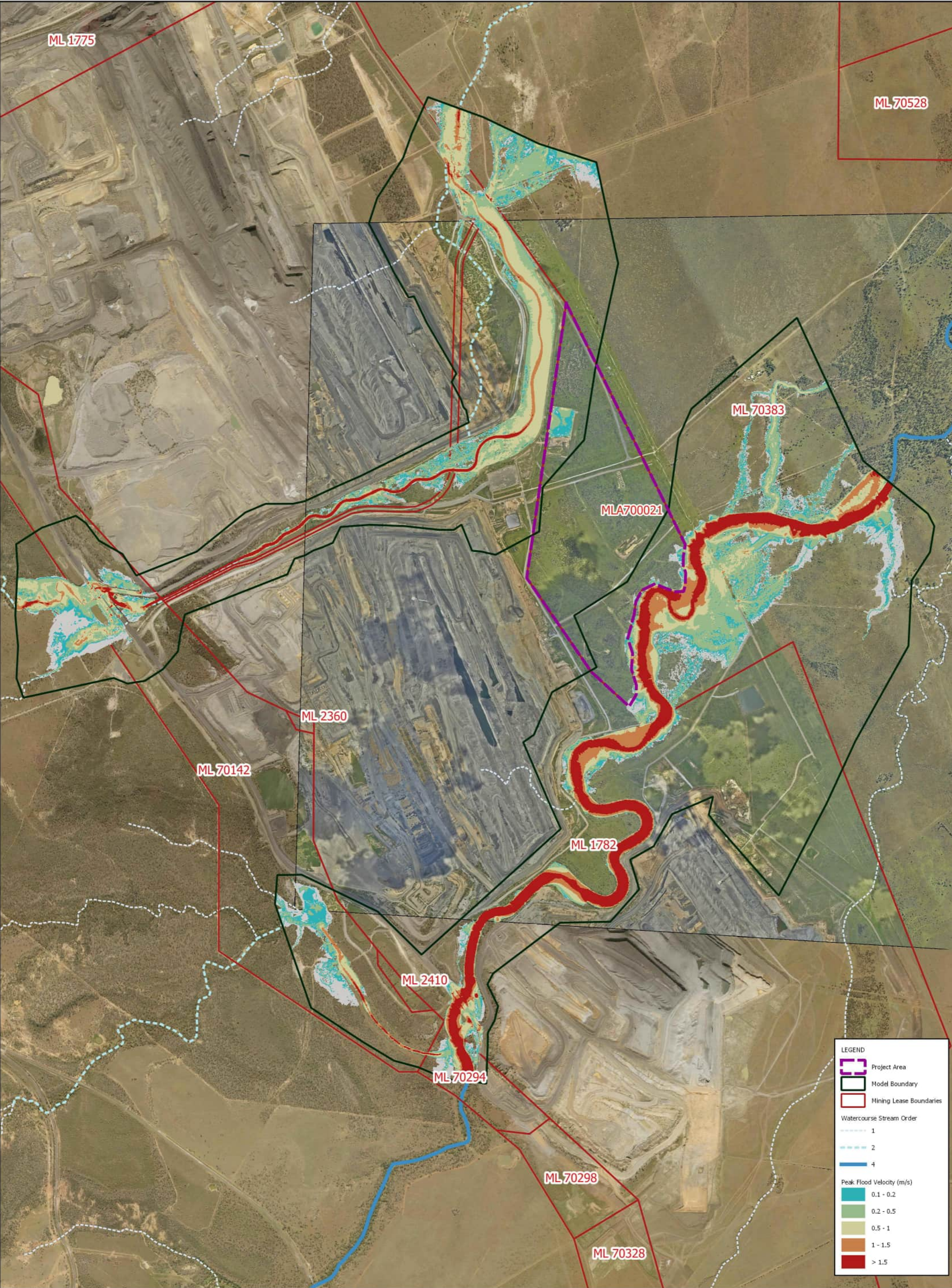
Figure 4 BM Alliance Coal Operations Pty Ltd Saraji Mine Grevillea Pit Continuation Project Surface Water Assessment Base Case 1% AEP Flood Velocity Drg Ref.
