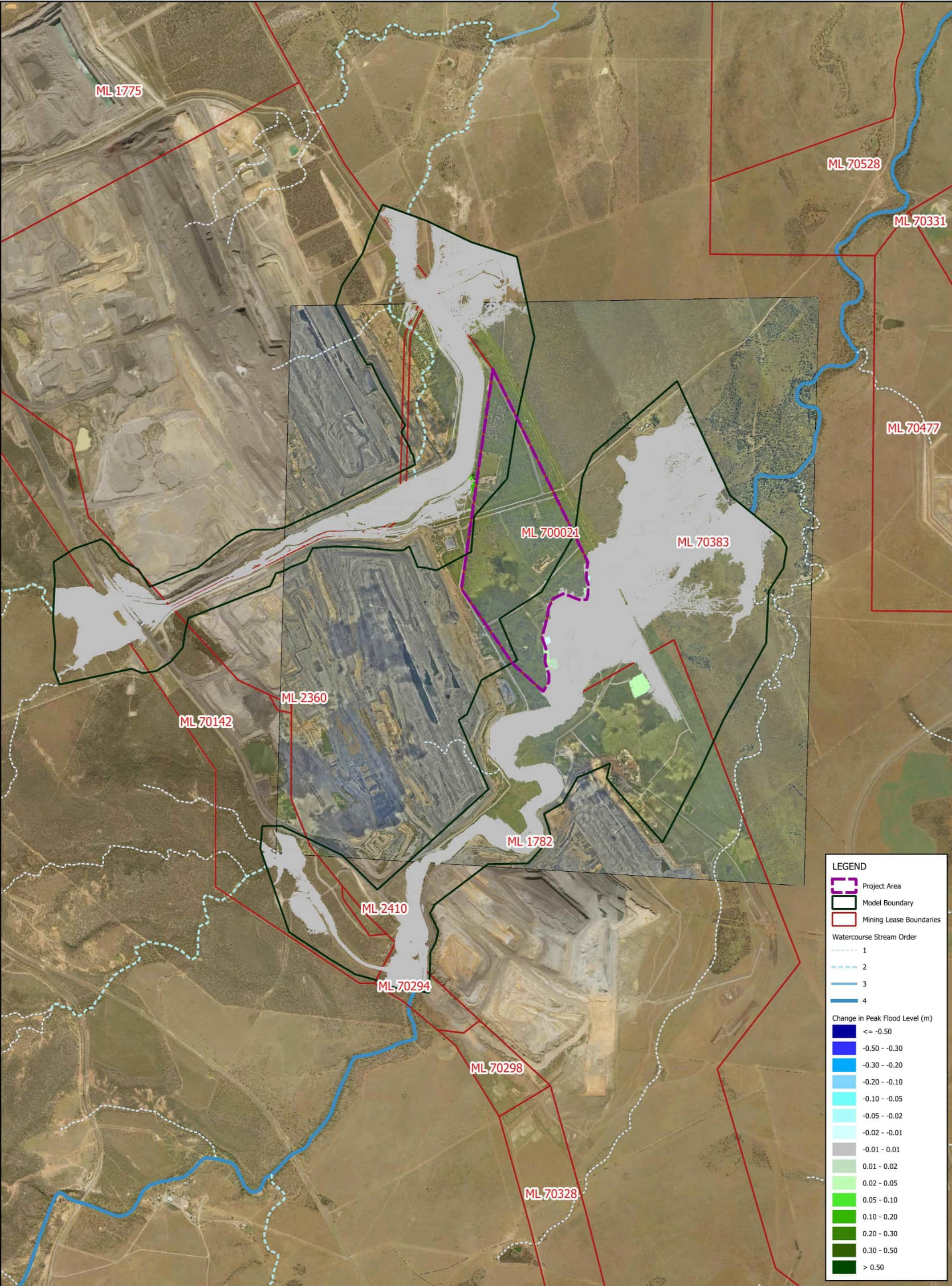
Figure 5 BM Alliance Coal Operations Pty Ltd Saraji Mine Grevillea Pit Continuation Project Surface Water Assessment Change in 1% AEP Flood Level Climate Change Sensitivity (SSP2-4.5) Drg Ref.
