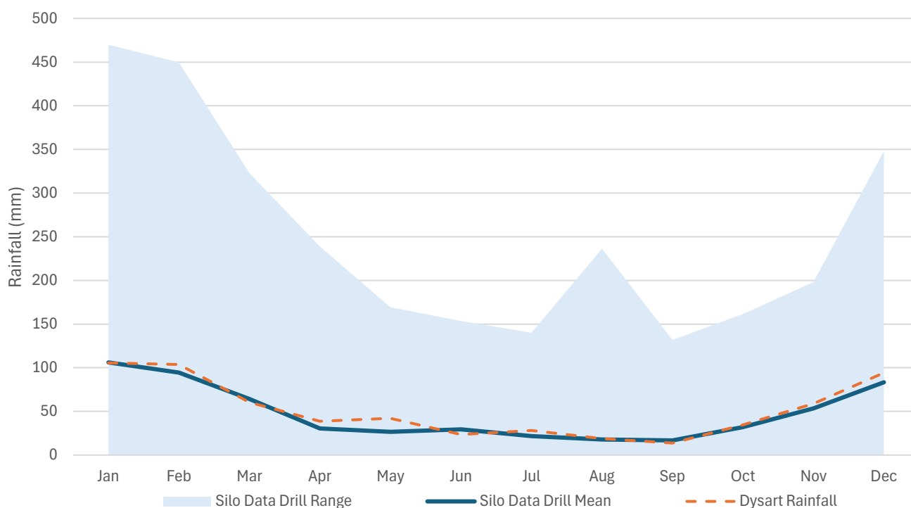
Figure 2.3: Monthly Rainfall
