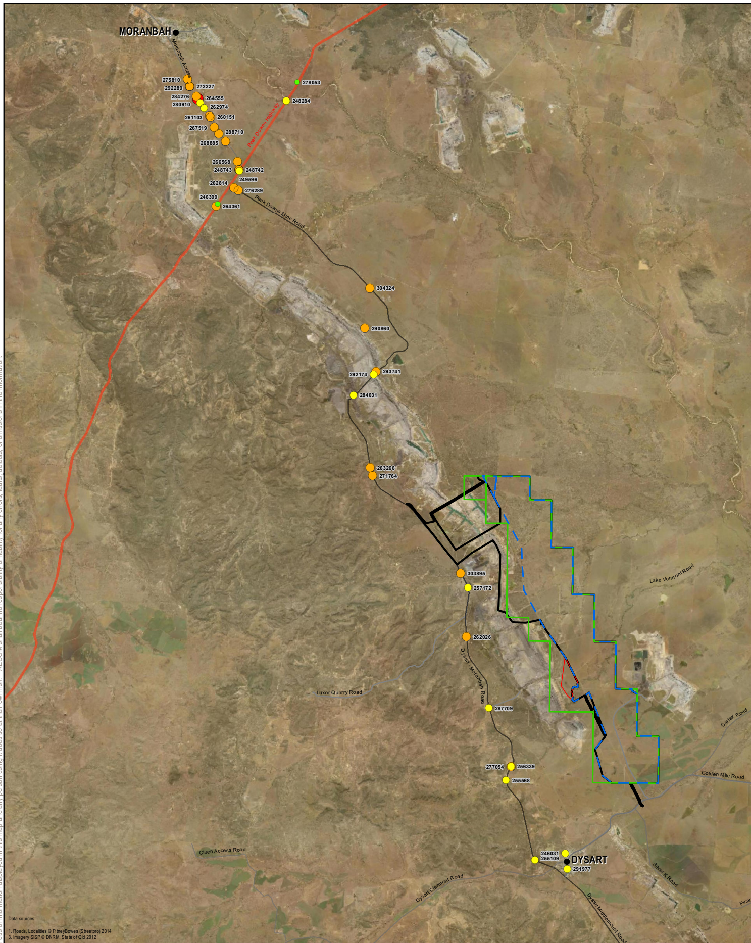
Figure 1 Crash Data
