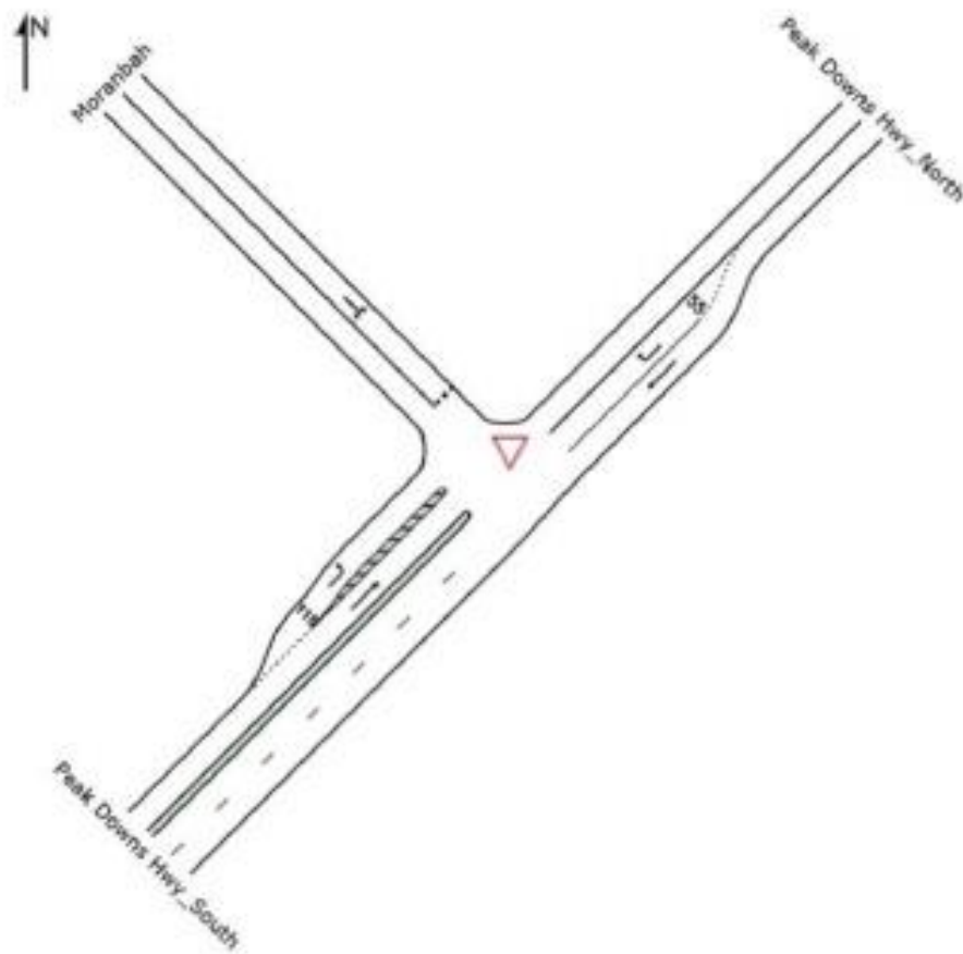
Figure 8 SIDRA layout for Intersection 5
