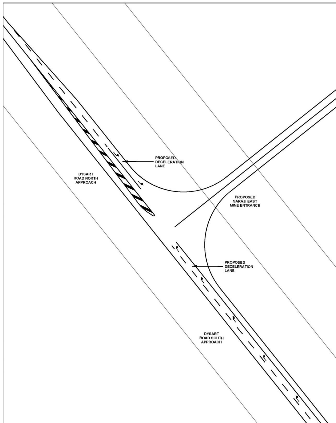
Figure 11 Concept Proposed Intersection A – Saraji Road / Saraji East Mine Entrance
