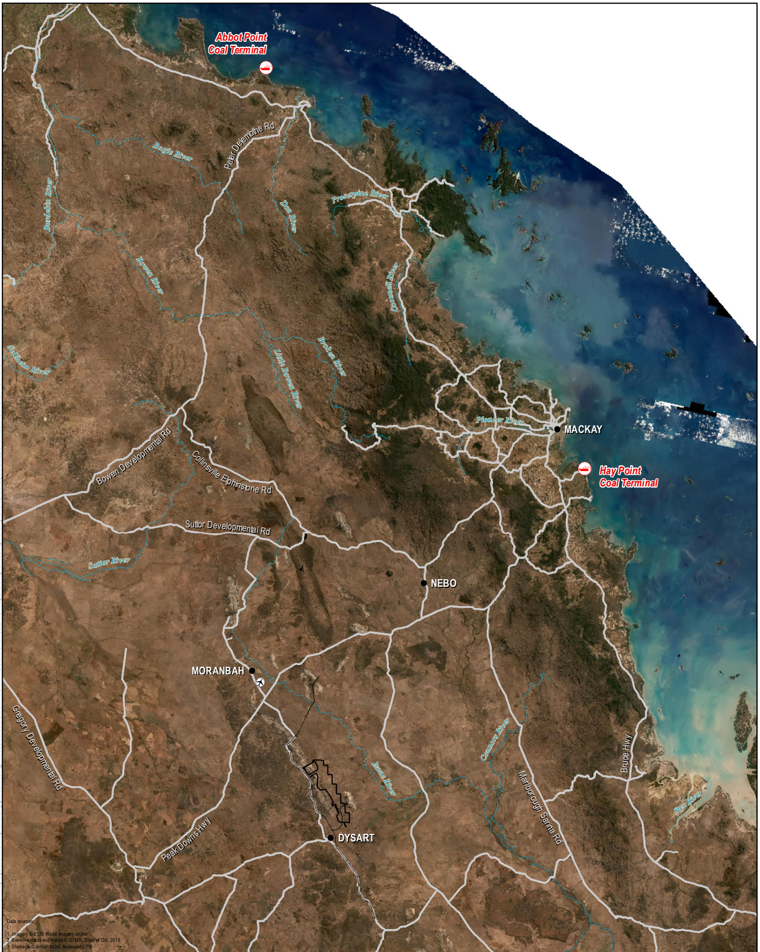
Figure 12 Coal terminals
