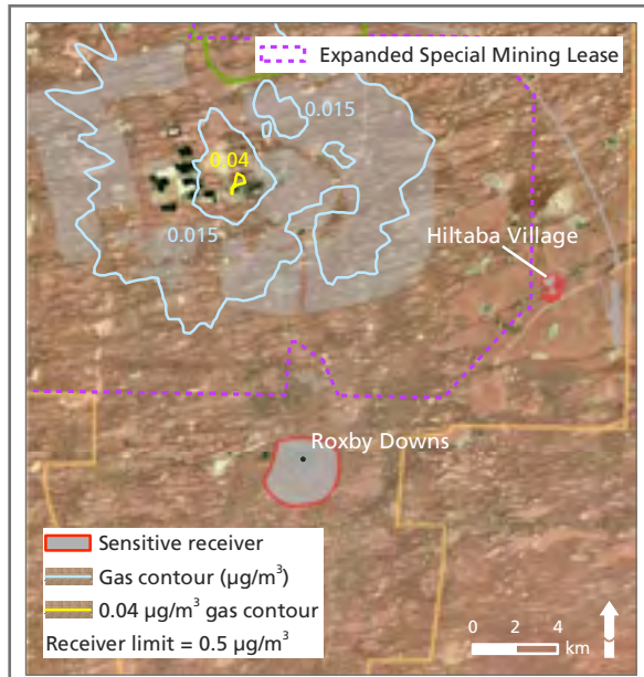
Figure G1.8 Predicted lead ground-level concentrations ( \mu\text{g}/\text{m}^3 )
