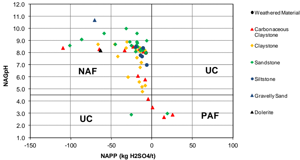
Figure 8: Geochemical Classification Plot for Selected Overburden and Interburden Samples from the Mt Arthur Coal Open Cut Modification.
