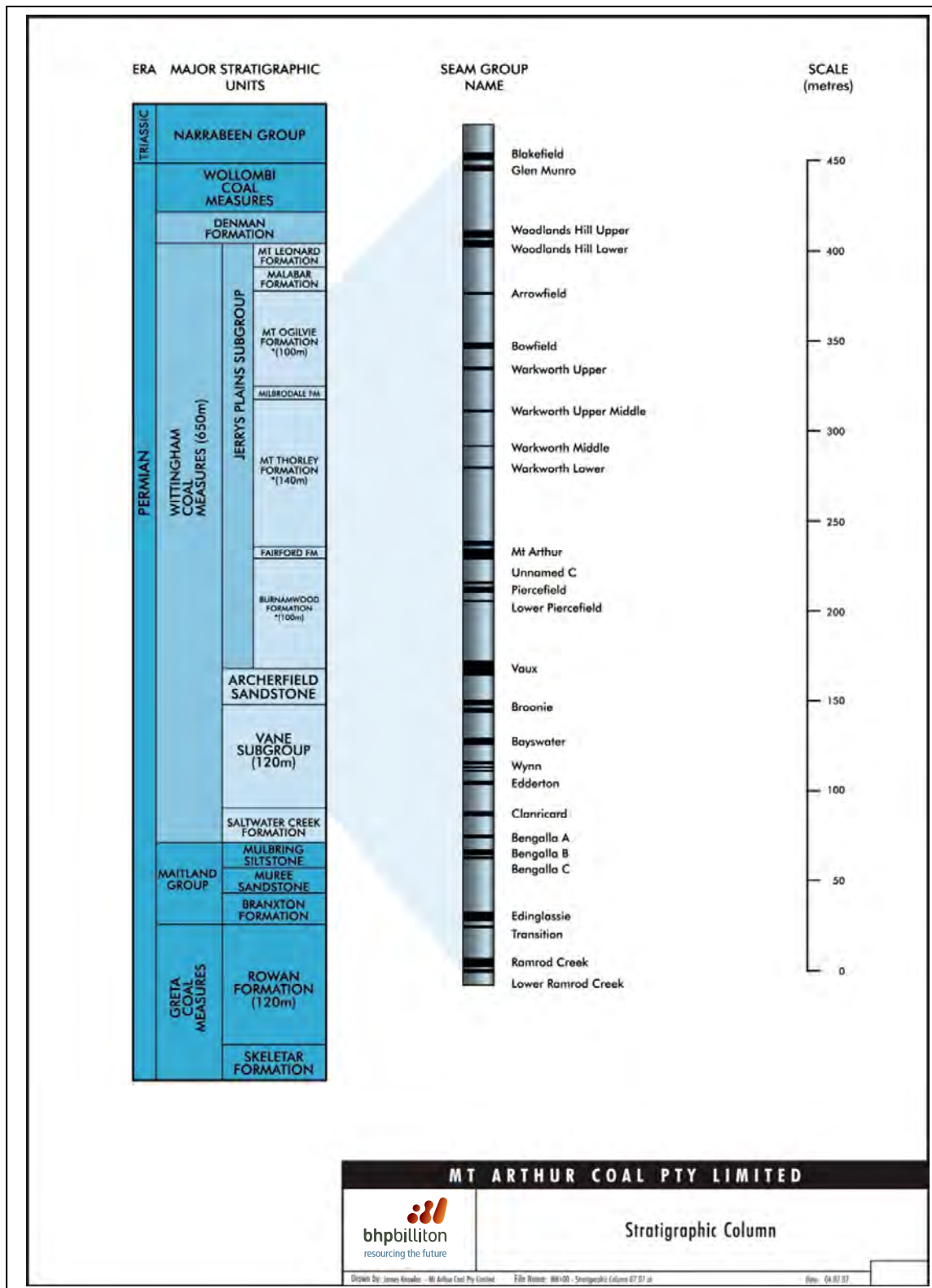
Figure 3: Stratigraphic Column for the Hunter Coalfield.
