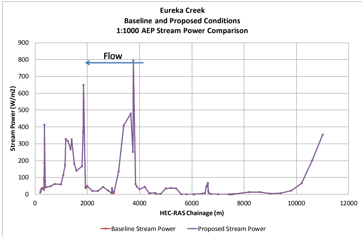
Figure Appendix E 33 Longitudinal Plot of Eureka Creek Stream Power Comparison 1 in 1000 AEP
