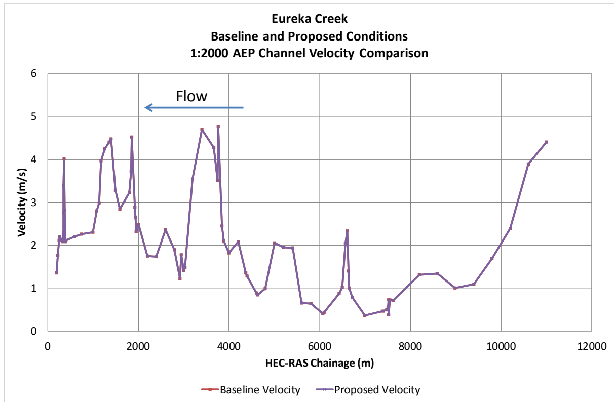
Figure Appendix E 35 Longitudinal Plot of Eureka Creek Stream Velocity Comparison 1 in 2000 AEP
