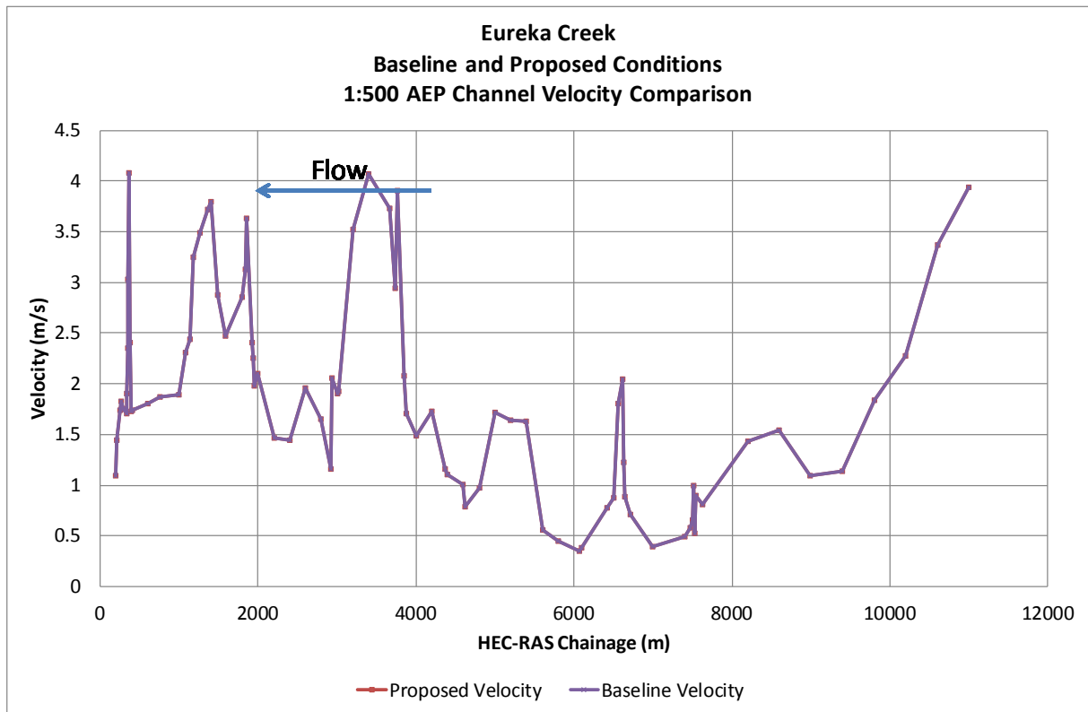
Figure Appendix E 29 Longitudinal Plot of Eureka Creek Stream Velocity Comparison 1 in 500 AEP
