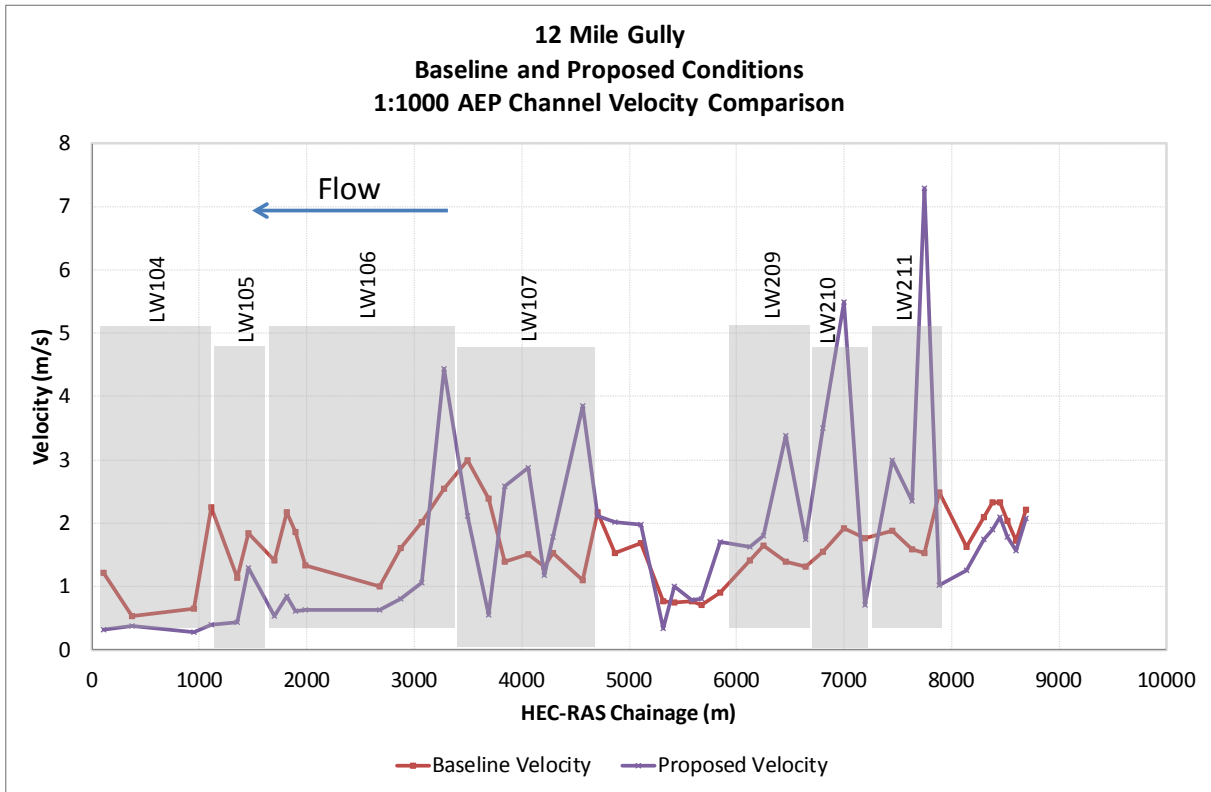
Figure Appendix E 8 Longitudinal Plot of 12 Mile Gully Stream Velocity Comparison 1 in 1000 AEP
