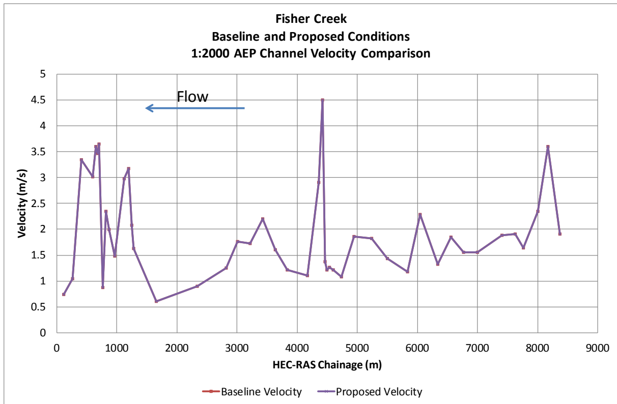
Figure Appendix E 47 Longitudinal Plot of Fisher Creek Stream Velocity Comparison 1 in 2000 AEP
