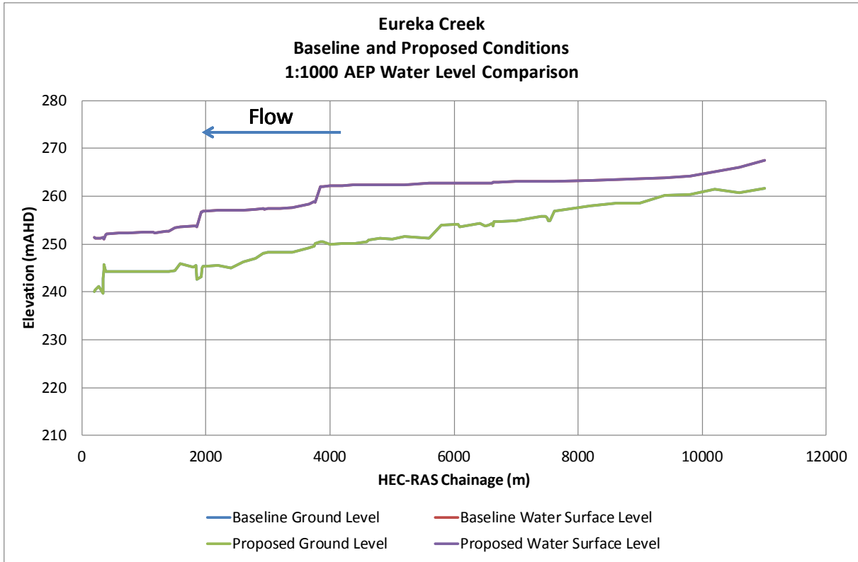
Figure Appendix E 31 Longitudinal Plot of Eureka Creek Water Surface Elevation Comparison 1 in 1000 AEP
