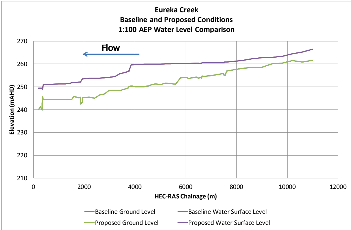
Figure Appendix E 25 Longitudinal Plot of Eureka Creek Water Surface Elevation Comparison 1 in 100 AEP
