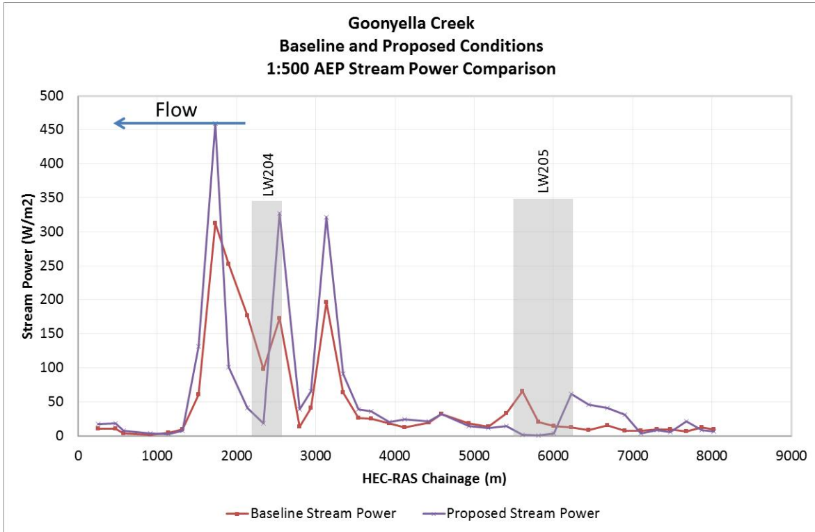
Figure Appendix E 18 Longitudinal Plot of Goonyella Creek Stream Power Comparison 1 in 500 AEP
