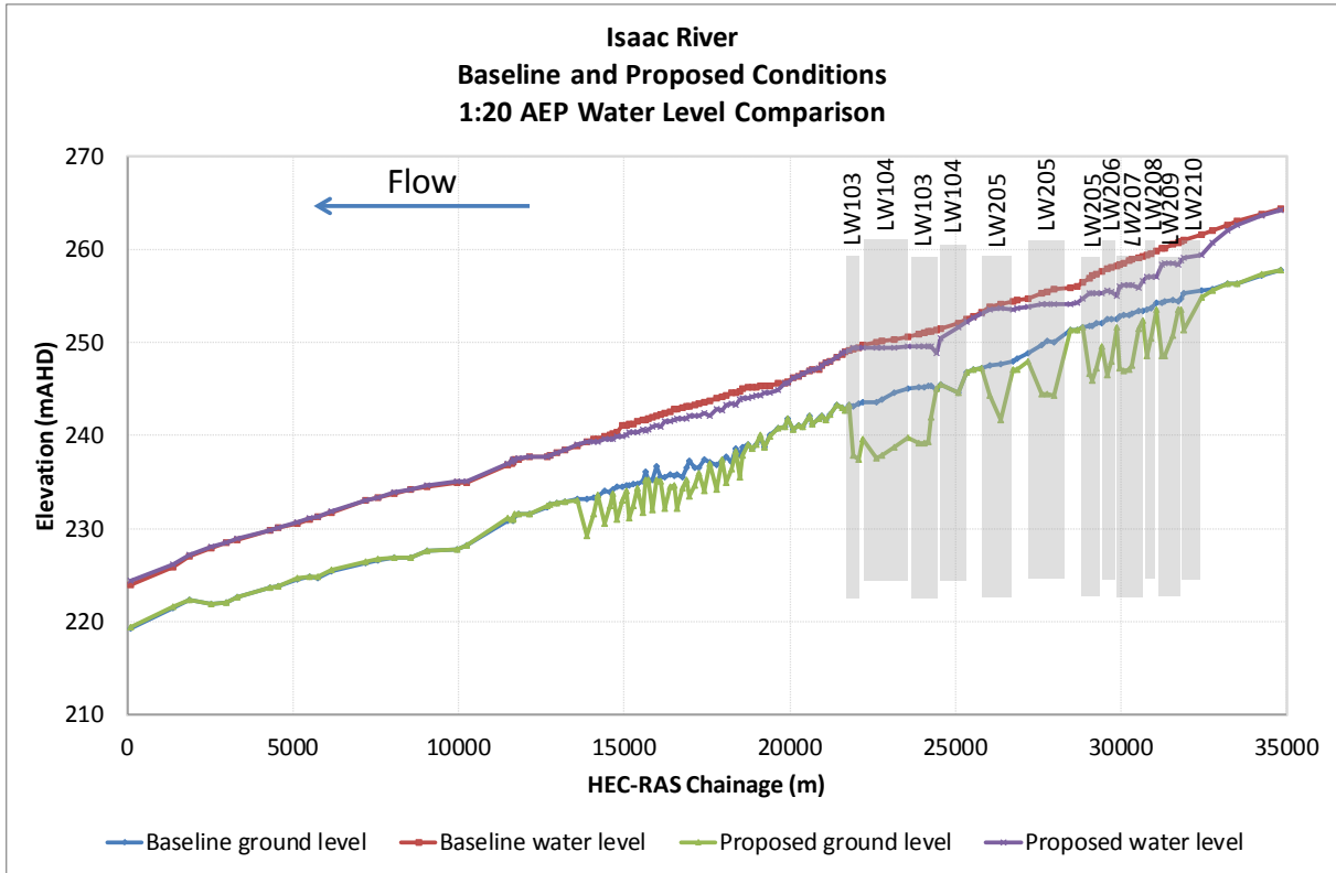
Figure Appendix C 4 Longitudinal Plot of Isaac River Water Surface Elevation Comparison 1 in 20 AEP
