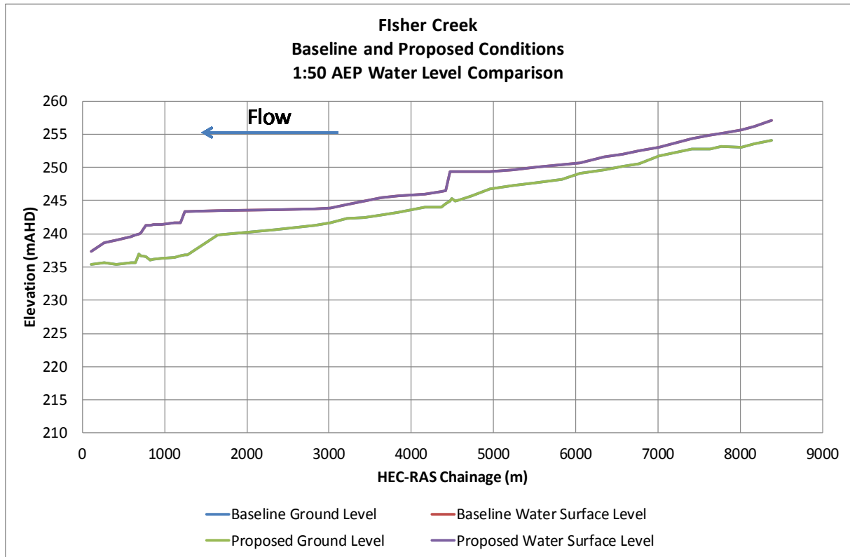
Figure Appendix C 43 Longitudinal Plot of Fisher Creek Water Surface Elevation Comparison 1 in 50 AEP
