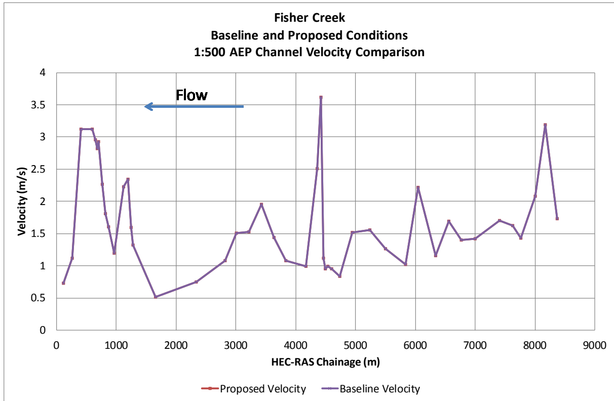
Figure Appendix E 41 Longitudinal Plot of Fisher Creek Stream Velocity Comparison 1 in 500 AEP
