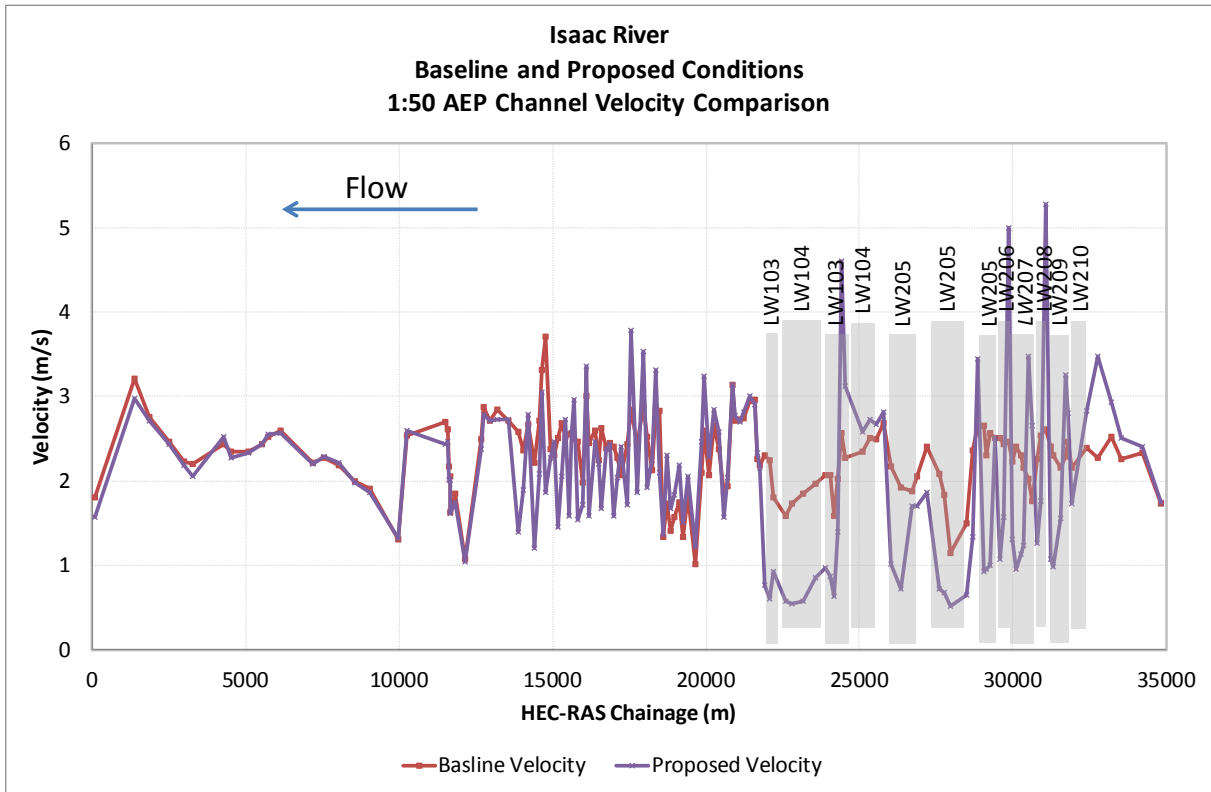
Figure Appendix C 8 Longitudinal Plot of Isaac River Stream Velocity Comparison 1 in 50 AEP
