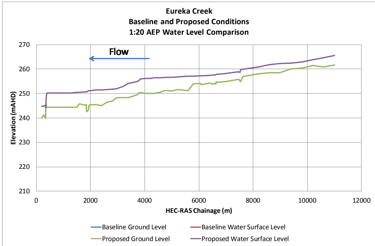
Figure Appendix C 31 Longitudinal Plot of Eureka Creek Water Surface Elevation Comparison 1 in 20 AEP
