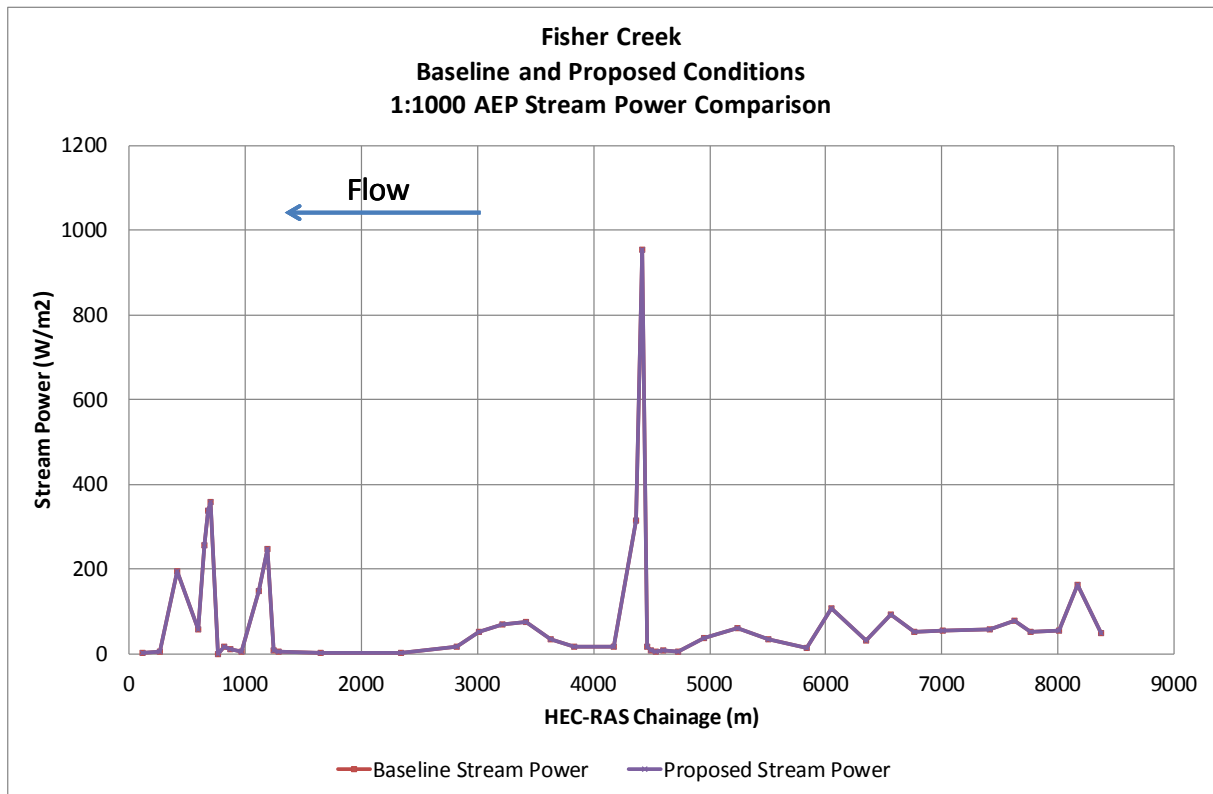
Figure Appendix E 45 Longitudinal Plot of Fisher Creek Stream Power Comparison 1 in 1000 AEP
