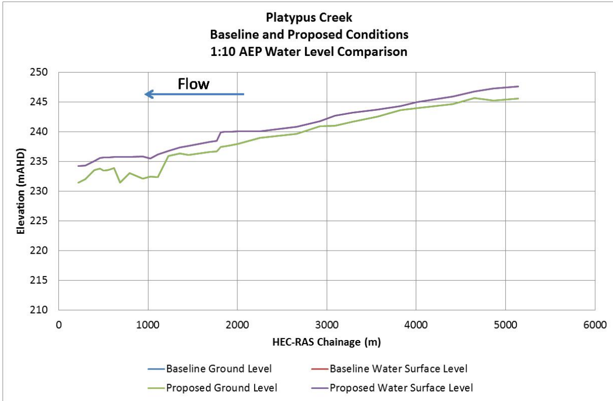
Figure Appendix C 46 Longitudinal Plot of Platypus Creek Water Surface Elevation Comparison 1 in 10 AEP
