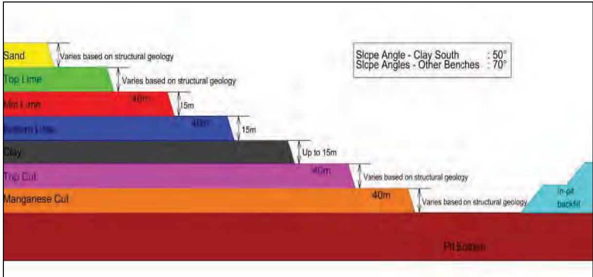
Figure 15 Schematic section through the pit, indicating cuts and thicknesses Source: Hotazel
