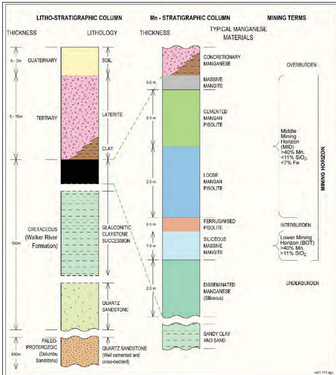
Figure 4 Stratigraphic column showing the manganese sequence
